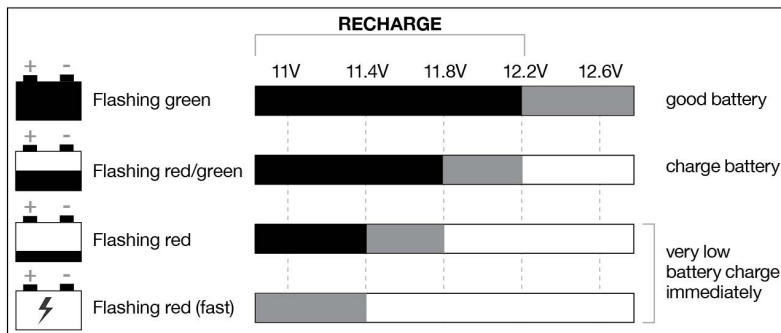
Fig. 4 BATTERY VOLTAGE
